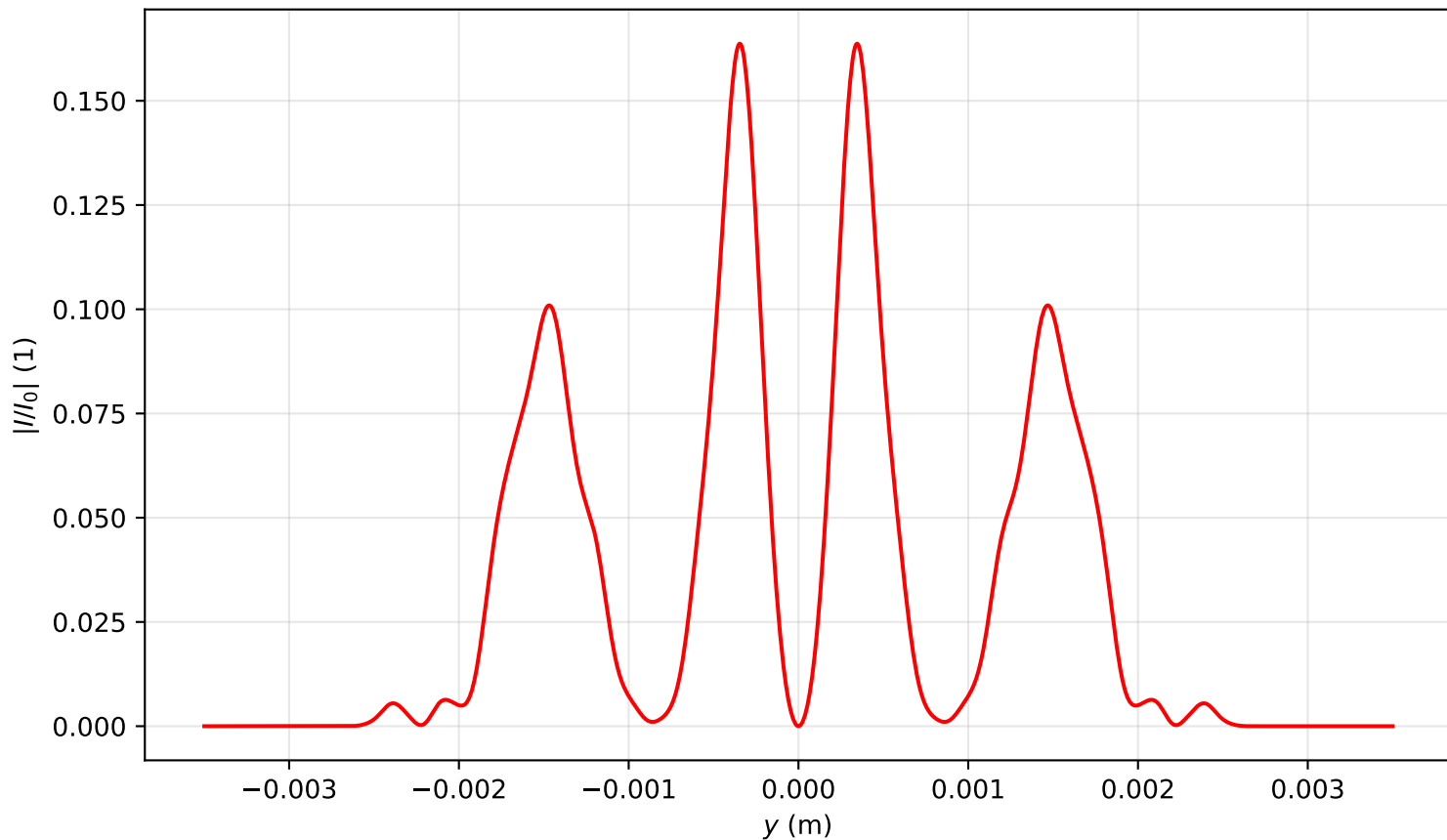
Intensity profile I(x=0, y, z=2.309)/I_0 , \text{Pin}=9.0\text{Pcr} , artificial time
